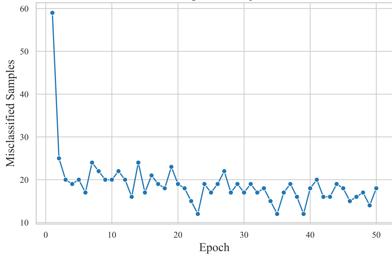
Training Error vs Epoch
